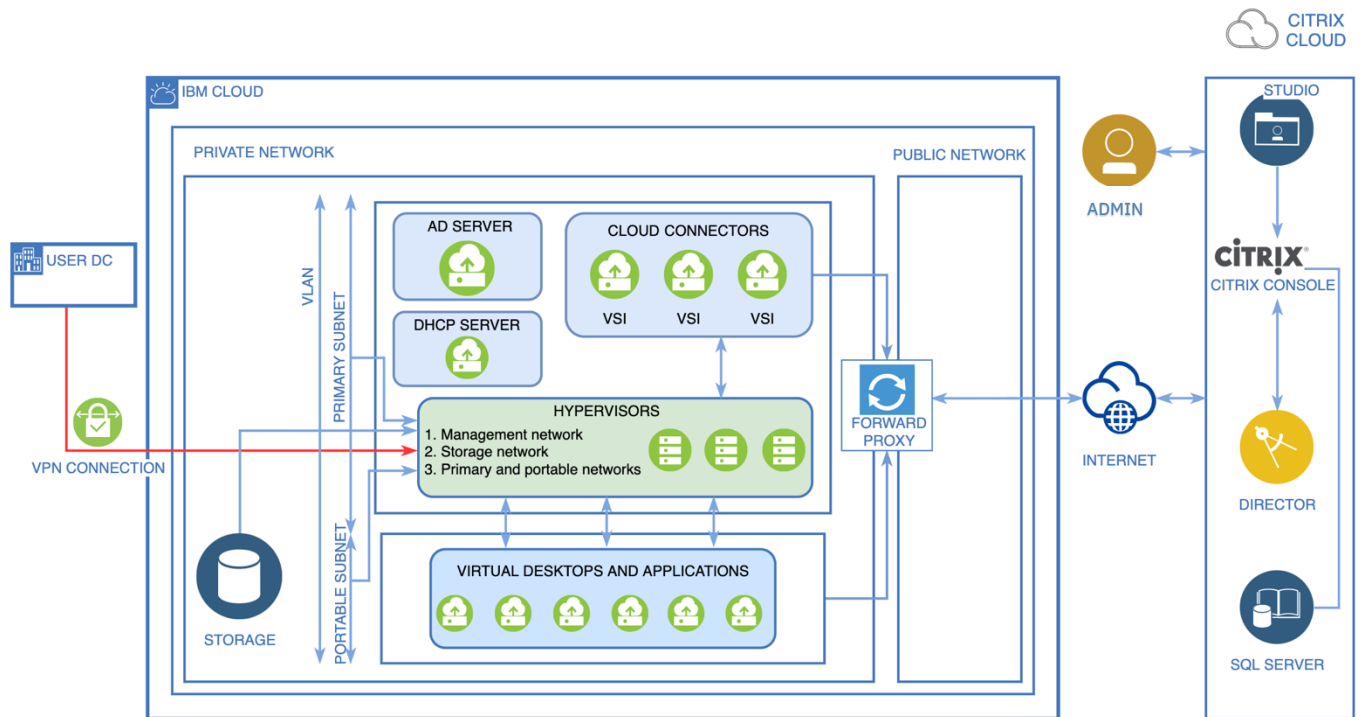
Figure 1: Citrix DaaS on IBM Cloud Architecture Diagram
